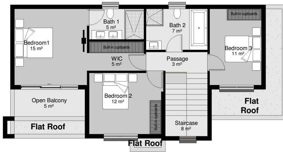
First Floor Plan (3 Bed )
