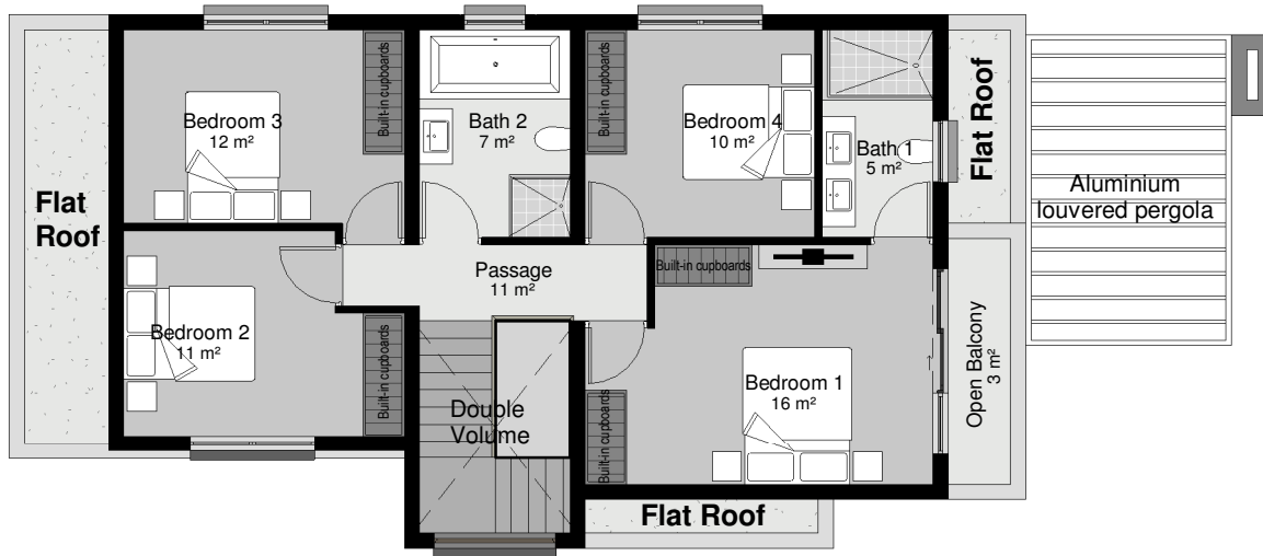
First Floor Plan (4 Bed)
