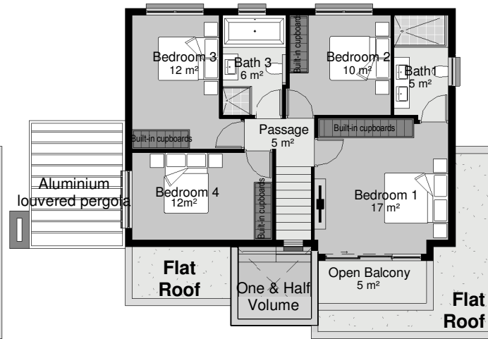
First Floor Plan (4 Bed)
