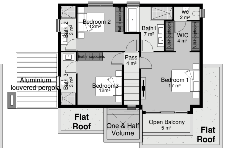
First Floor Plan (3 Bed 3 Ensuite)
