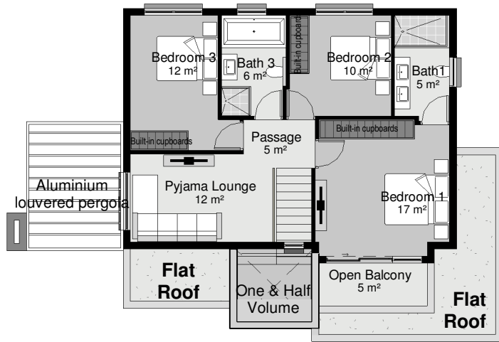
First Floor Plan (3B, PJ Lounge)
