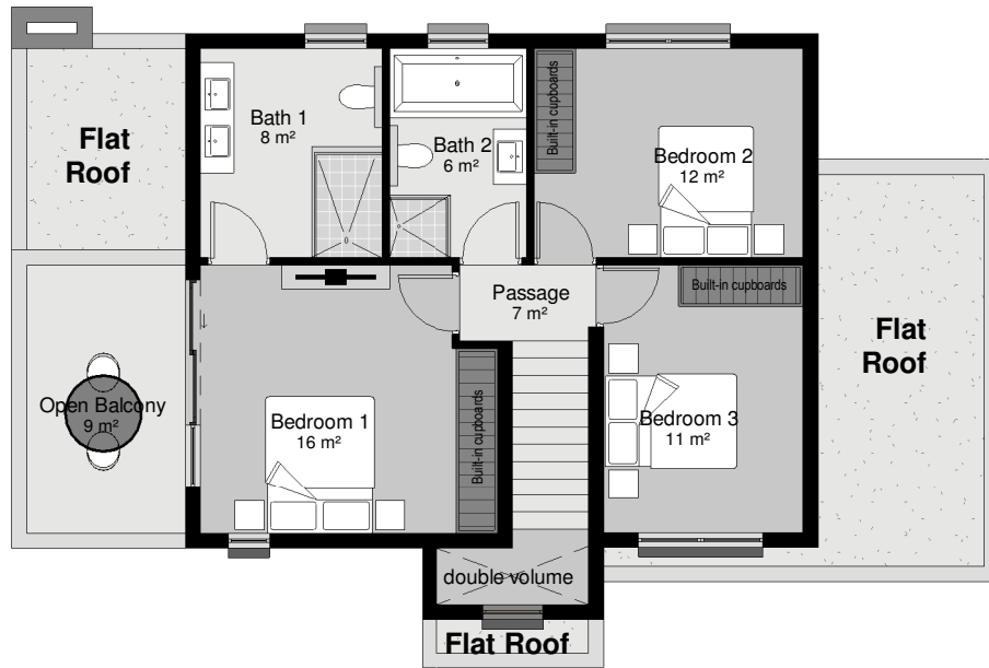
First Floor Plan (3 Bed )
